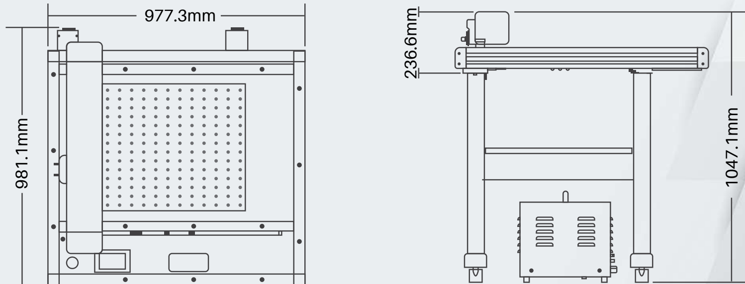
EXTERNAL DIMENSIONS
