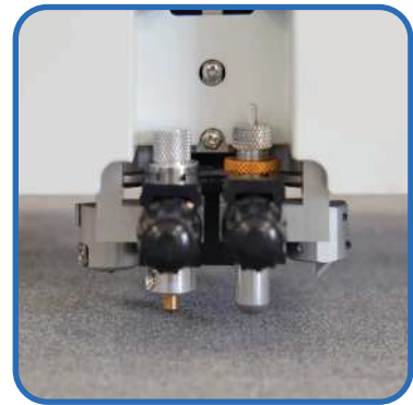
4 KNIFE HEAD DESIGN DIE-CUT+INDENTATION
