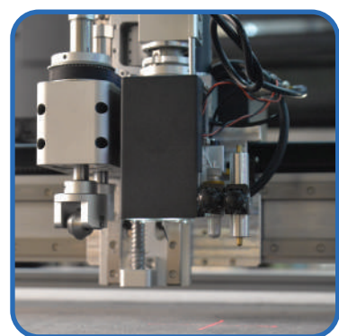
Five Knife Head Design
