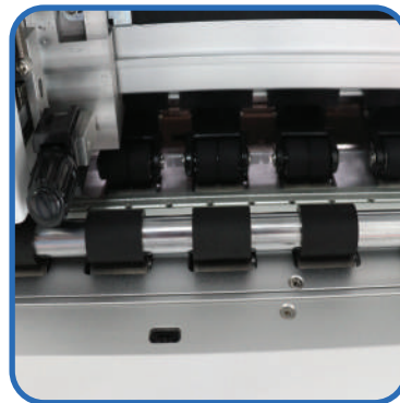
DOUBLE-PICKUP ROLLER
