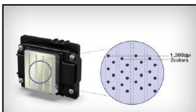
Single I3200-U1HD Heads
